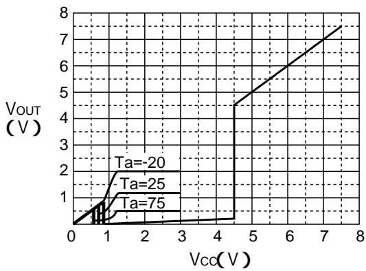
V CC vs. V OUT
