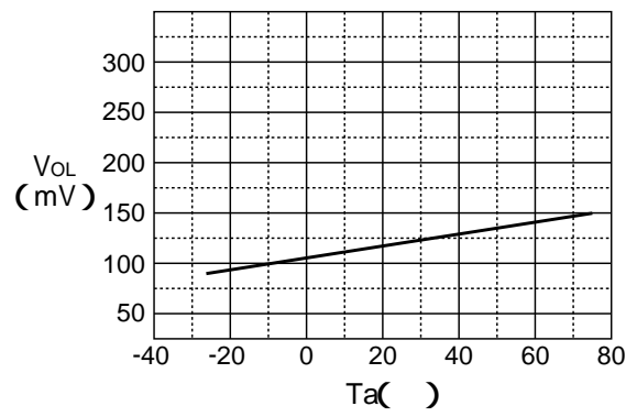
V OL vs. T a
