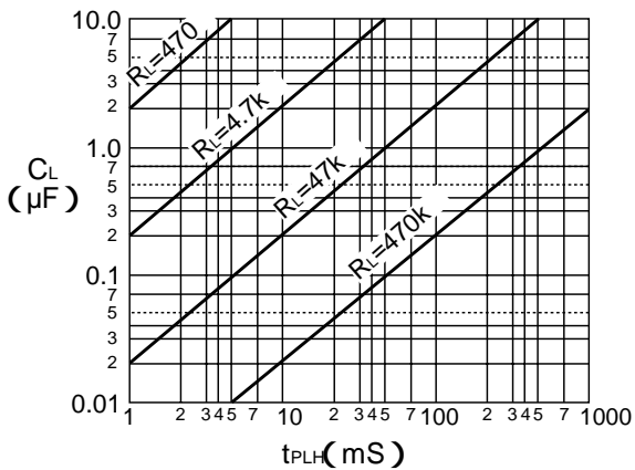
C L (R L ) vs. t PLH
